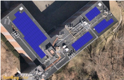
On-site renewables include a proposed 23.9 kW rooftop array (top left) or a 63 kW rooftop array (bottom left) in addition to the existing 120-panel 27.6 kW ground array located on site (right).
